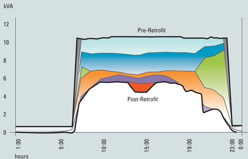
Colored areas between the respective load profiles (Pre-retrofit and Post-retrofit) represent typical energy savings from each strategy over a 24 hour period, averaged over 1 hour intervals.
